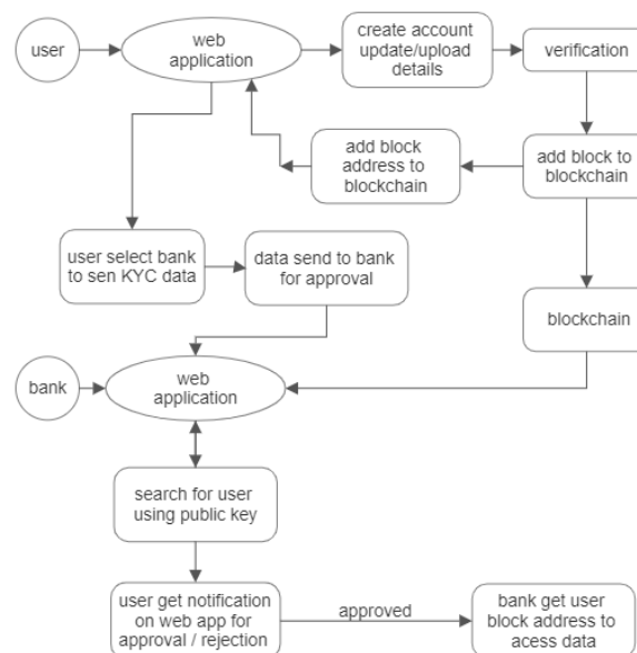
Figure 3: System Architecture Diagram
