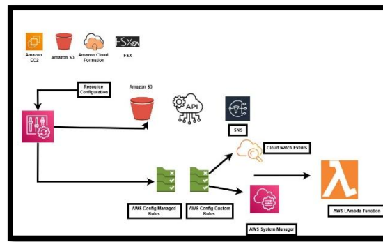
Fig 3: AWS Config Rule Architecture
